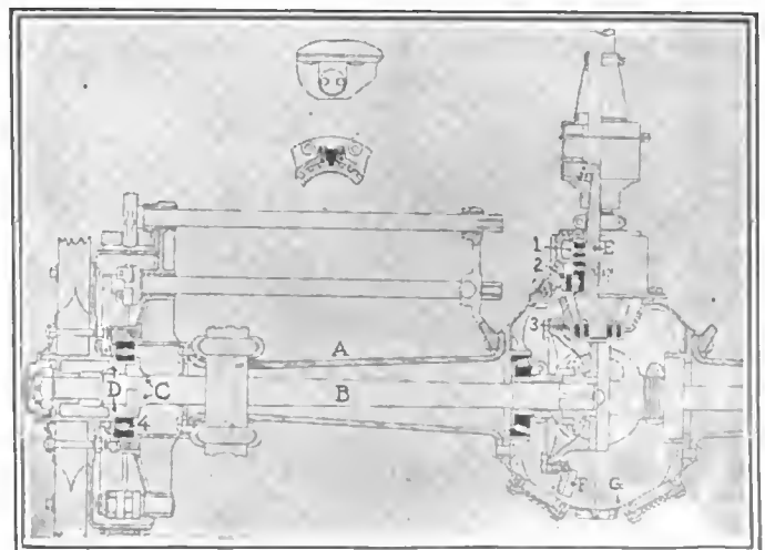
Fig. 6—The patented rear axle on the Premier
